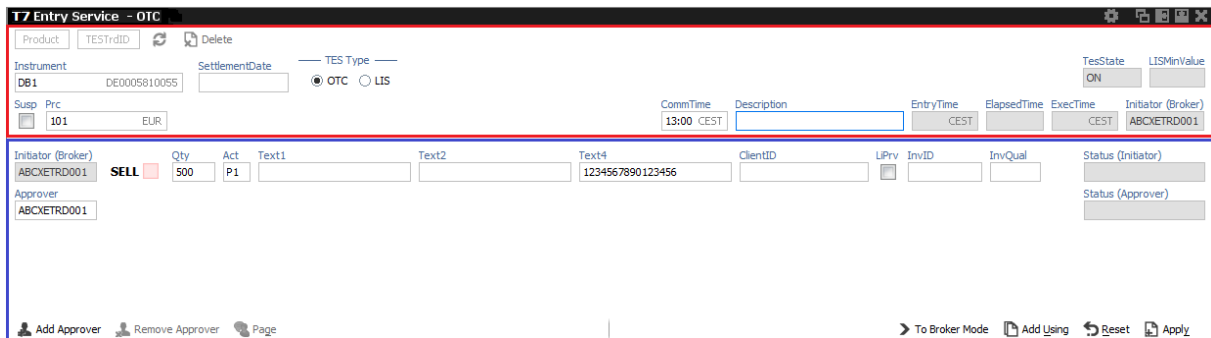
Fig. 64: Screenshot of TES Entry view in Simple Mode highlighting tradeable section and counterparty section
