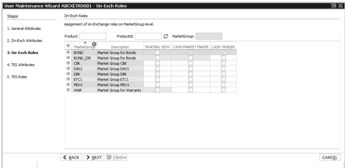
Fig. 100: Screenshot of the User Maintenance Wizard showing the entitlement roles on the On-Exch Roles tab
