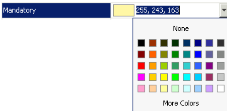
Fig. 16: Color Chooser
