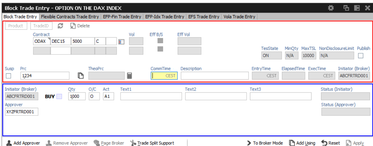
Fig. 77: Screenshot of the TES Entry view in Simple Mode
