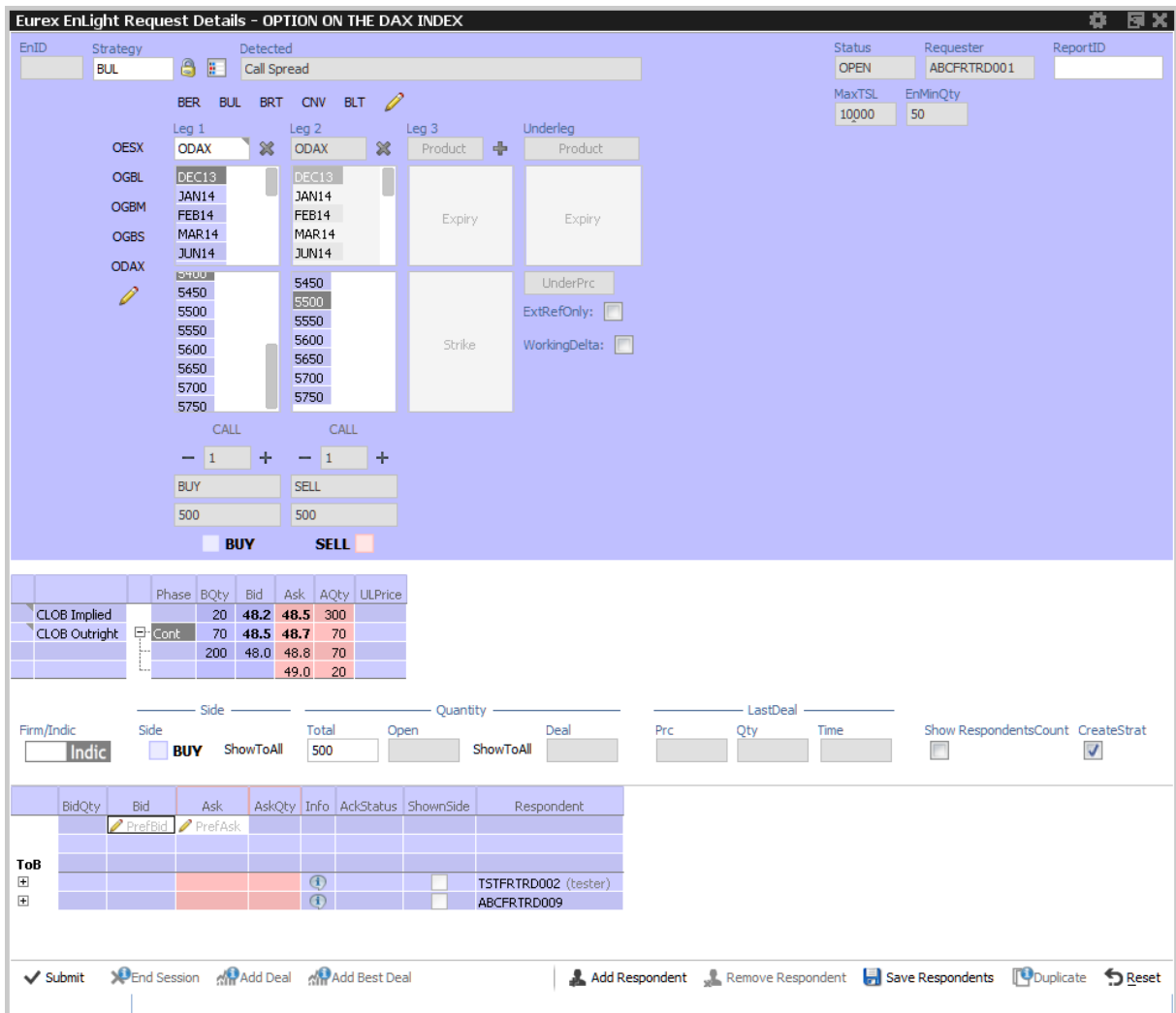
Fig. 101: Screenshot of the Eurex EnLight Request Details view showing a BUL strategy and new CLOB data display
