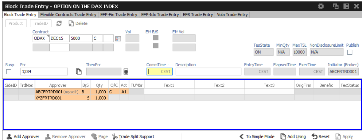
Fig. 78: Screenshot of the TES Entry view in Broker Mode
