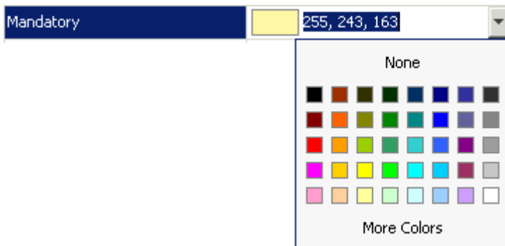
Fig. 18: Color Chooser
