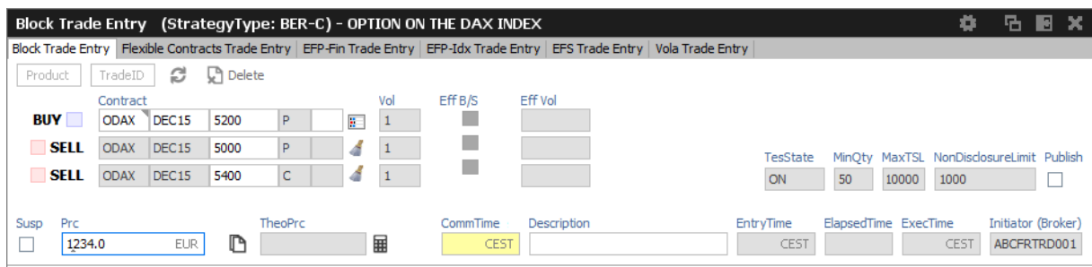
Fig. 86: Screenshot of the TES - Block Trade Entry view for a strategy
