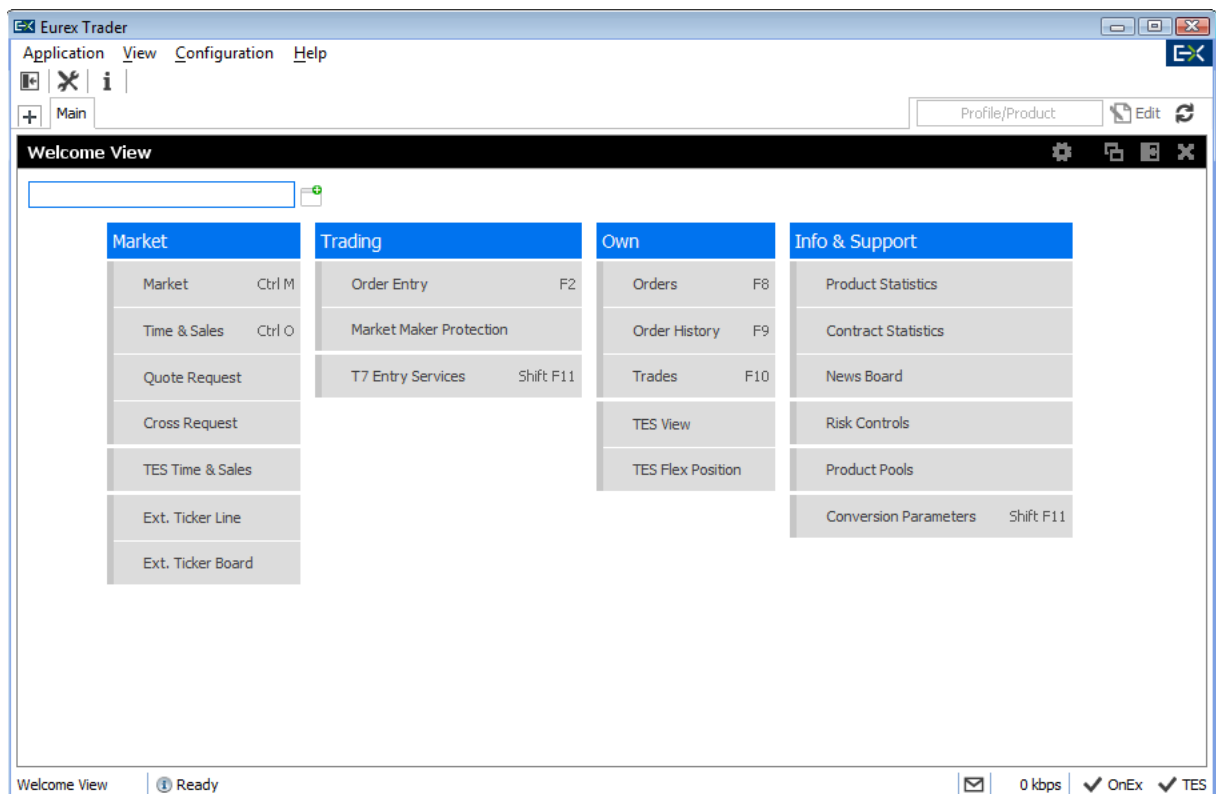
Fig. 50: Screenshot of Eurex Trader showing the Welcome view
