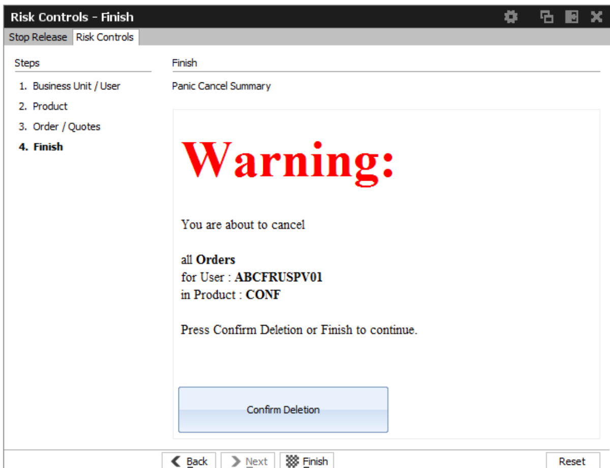
Fig. 111: Screenshot of the Risk Controls , showing step 4 of Panic Cancel
