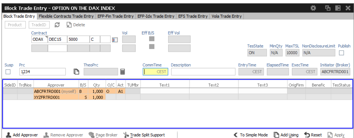
Fig. 75: Screenshot of the TES Entry view in Broker Mode
