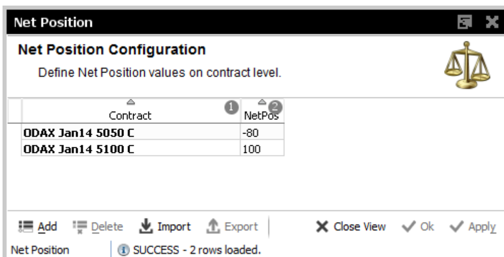
Fig. 53: Screenshot of the Net Position Configuration view
