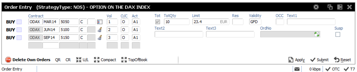
Fig. 69: Screenshot of the Order Entry showing the entry of a non standard options strategy.
