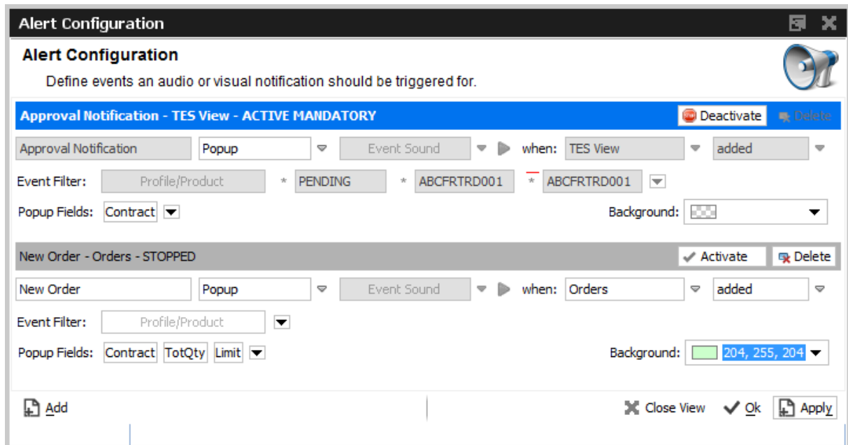
Fig. 52: Screenshot of the Alert Configuration view
