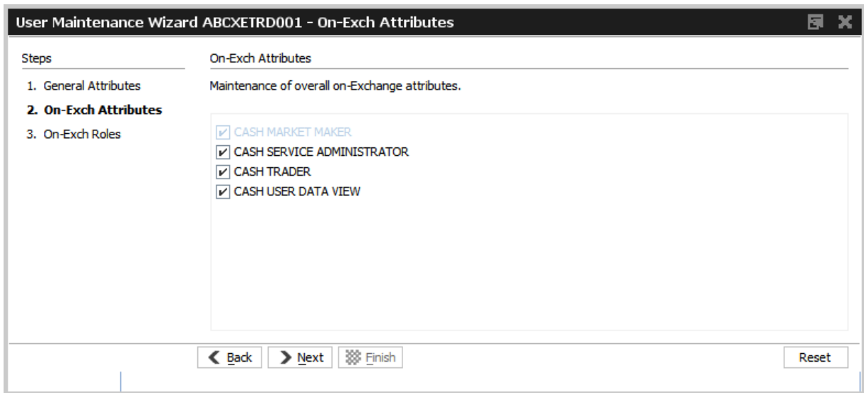
Fig. 69: Screenshot of the User Maintenance Wizard showing the Attributes tab
