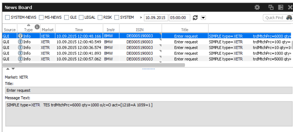
Fig. 64: Screenshot of the News Board view
