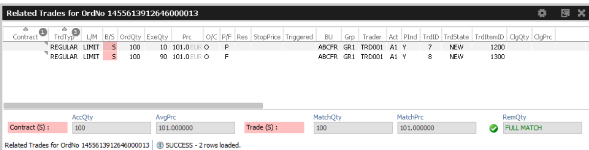
Fig. 62: Screenshots showing how to open the Related Trades view from the Trades or Orders view
